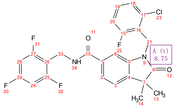
PC-7336801, DMSO-d6
